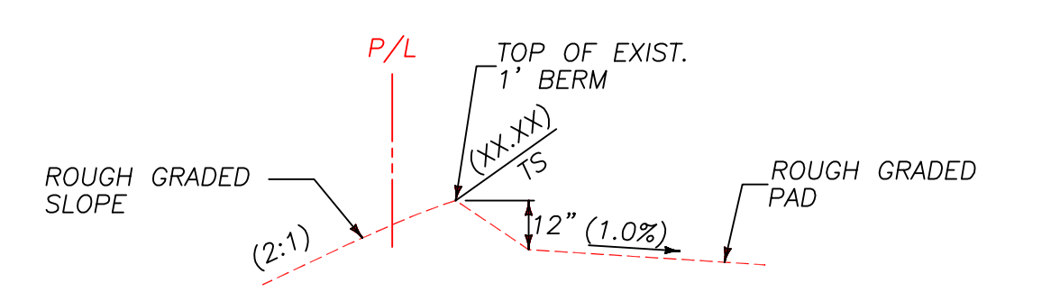
TYPICAL SECTION PER APPROVED ROUGH GRADING PLAN FOR REAR YARDS SLOPES GREATER THAN 5' IN VERTICAL HEIGHT NOT TO SCALE
