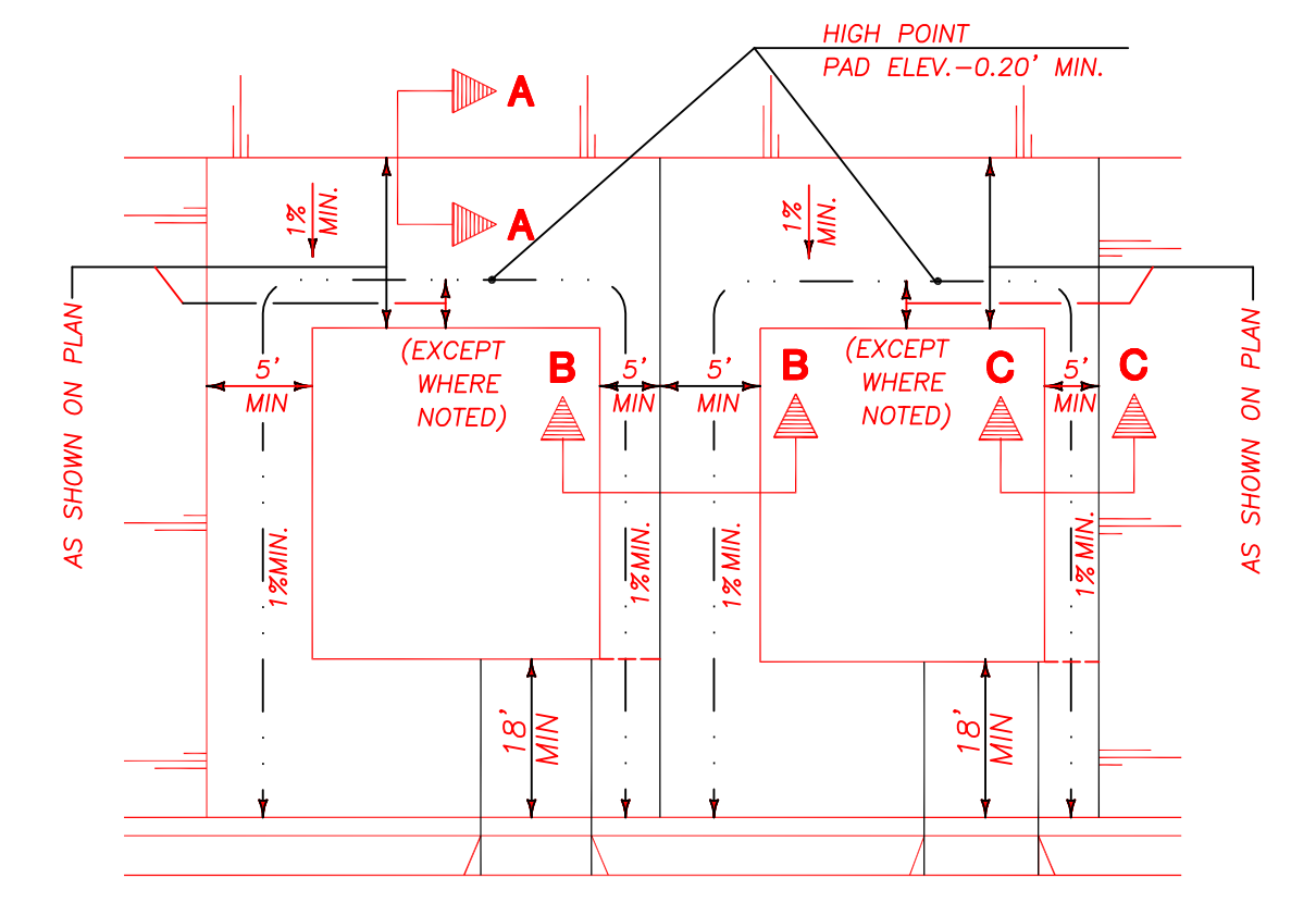
TYP. SIDE YARD DRAINAGE DETAIL NOT TO SCALE
